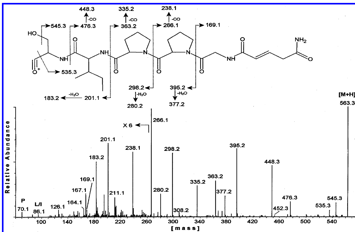
Figure 2. Sequence assignment Ser-Ile-Pro-Pro-Gly-Gln from the nozzle/skimmer fragmentation of the daughter ion at 563.3 mass units in the TOF MS/MS of the molecular ion [M + H]^+ of 1 .
